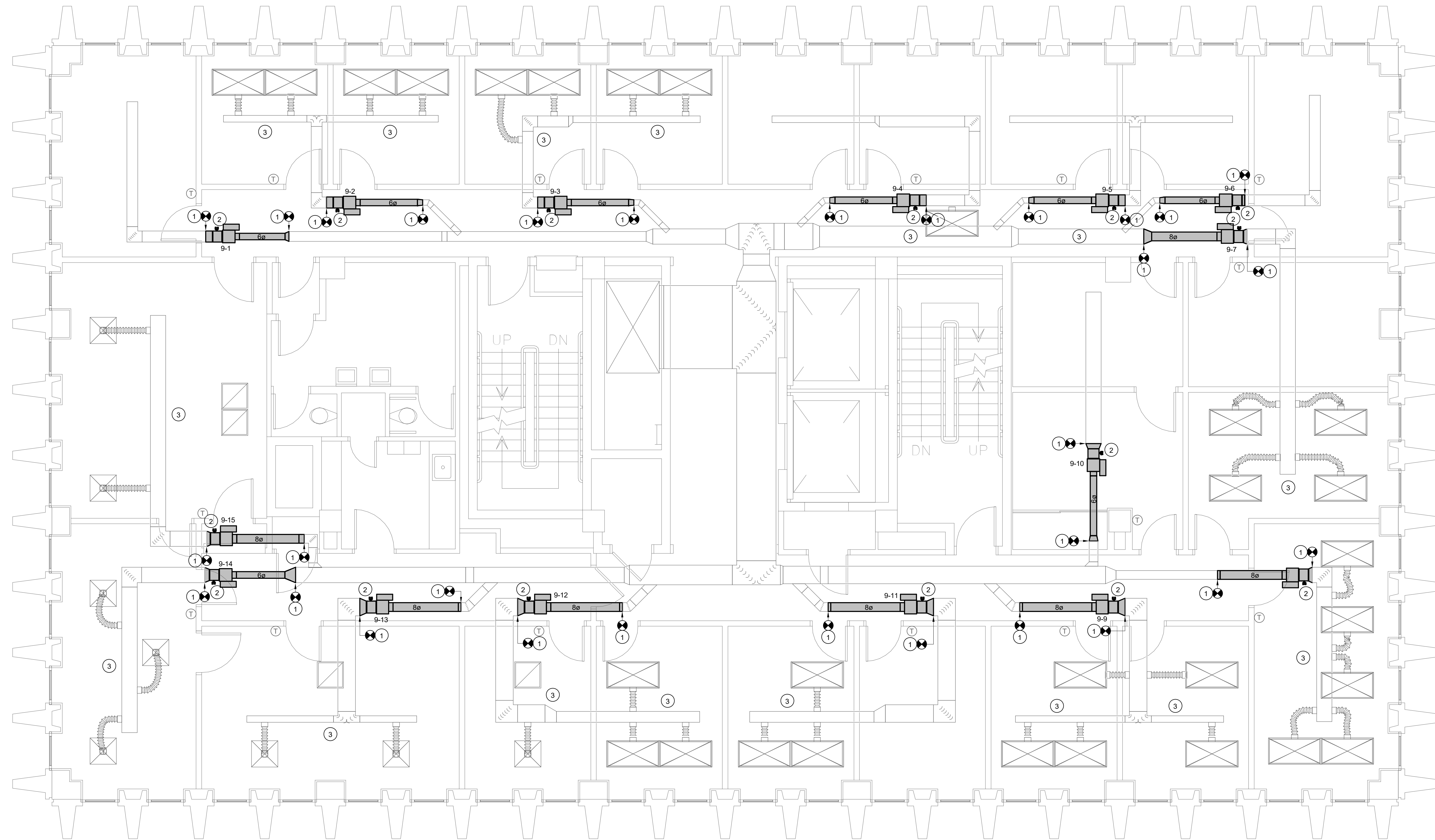
1 NINTH FLOOR RENOVATION PLAN M6 1/4" = 1'-0"
