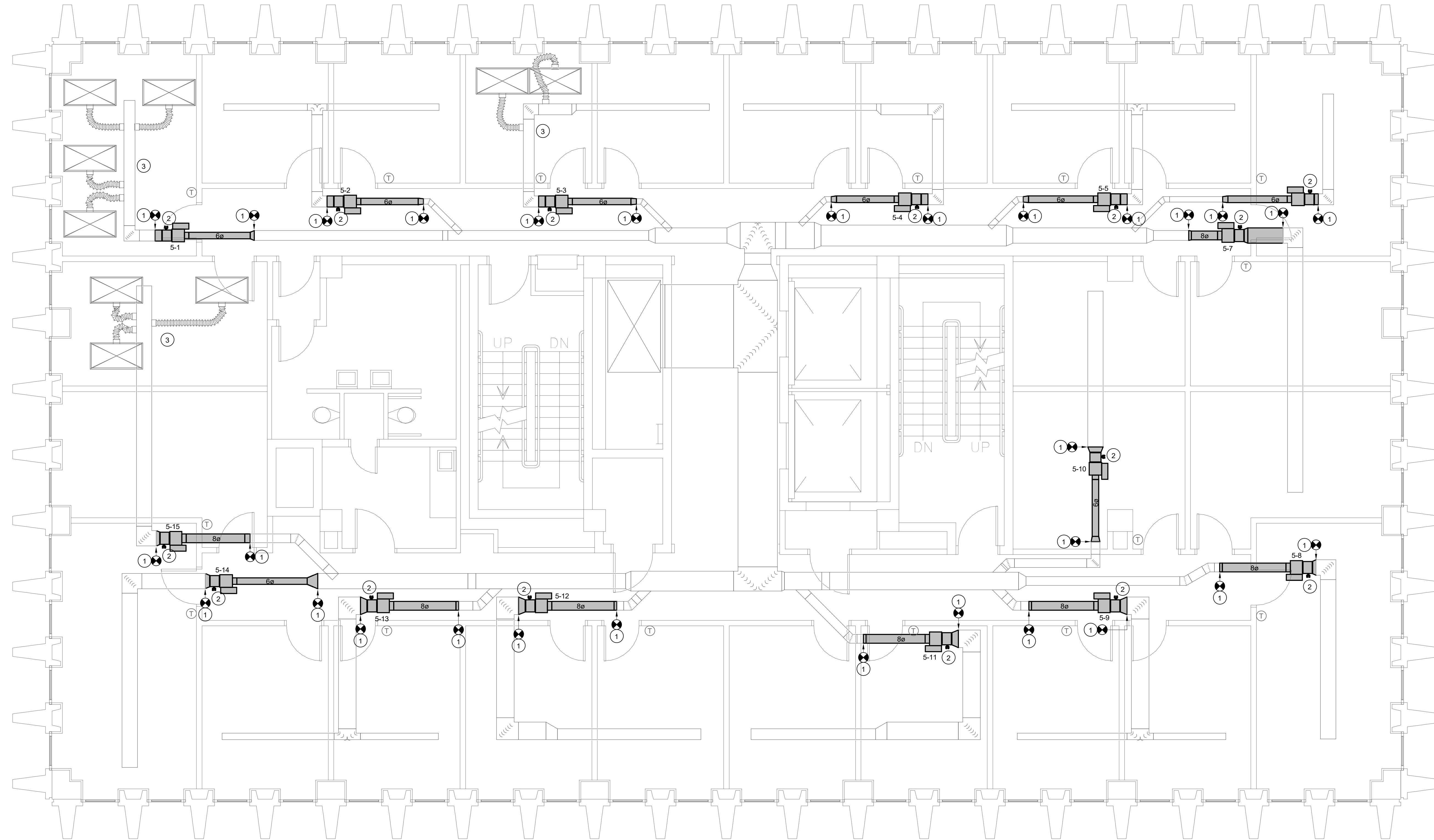
1 FIFTH FLOOR RENOVATION PLAN (ALTERNATE 1) M2 1/4" = 1'-0"
