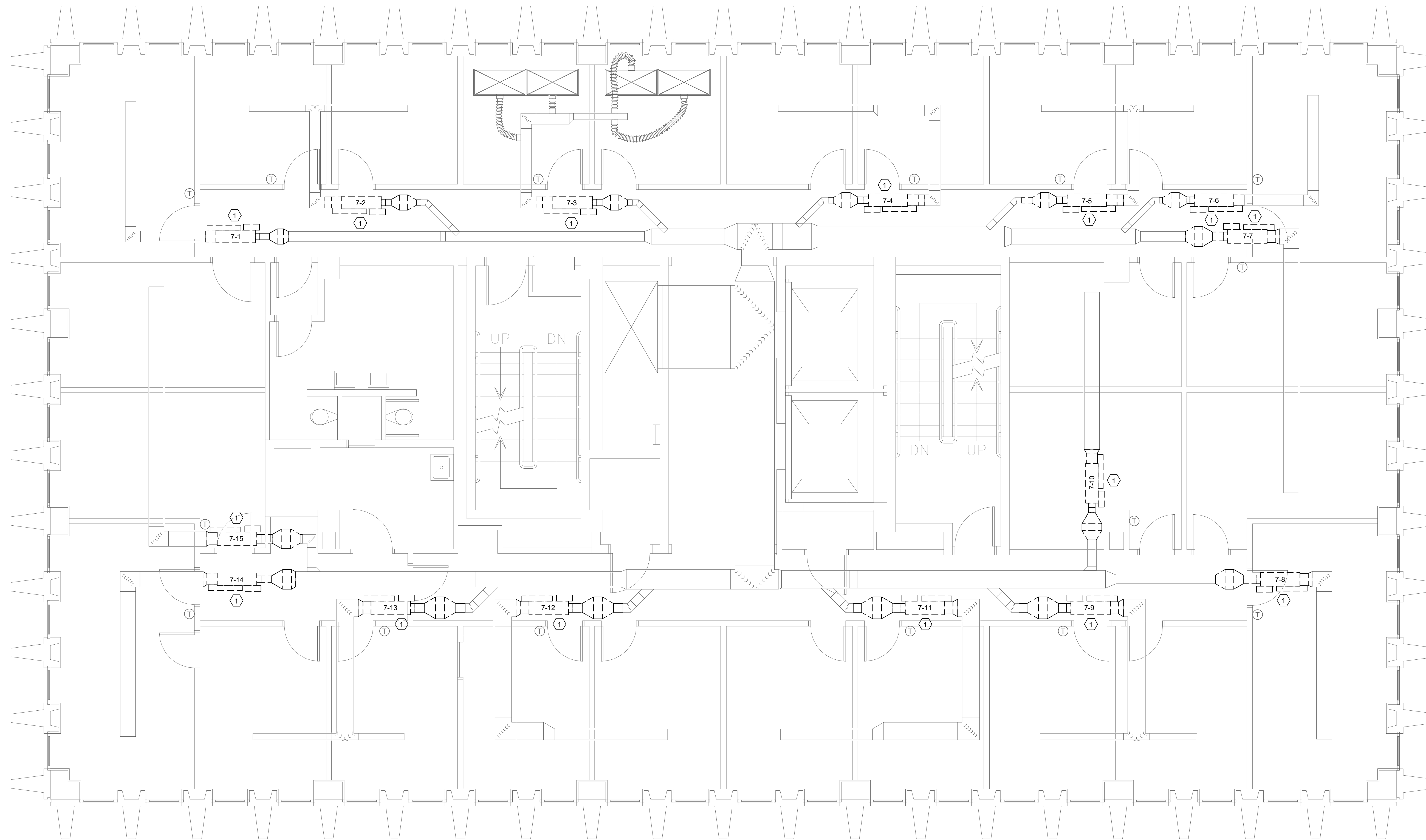
① SEVENTH FLOOR DEMOLITION PLAN MD4 1/4" = 1'-0"
