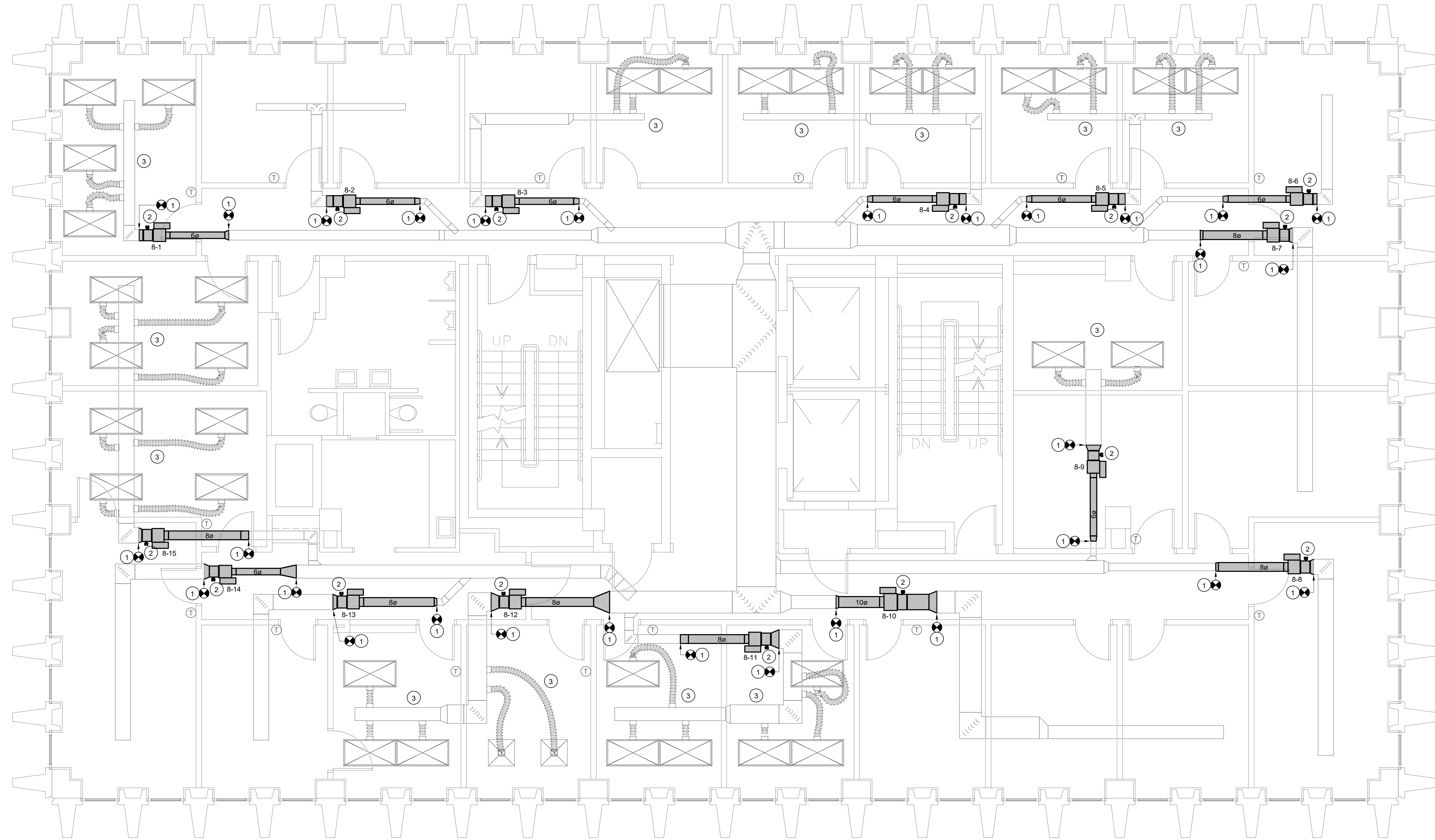
1 EIGHTH FLOOR RENOVATION PLAN M5 1/4" = 1'-0"
