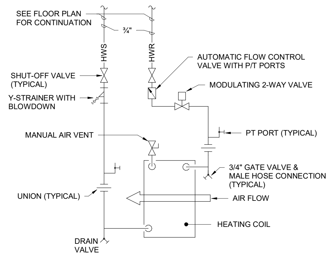
VAV HEATING COIL PIPING DETAIL NO SCALE
