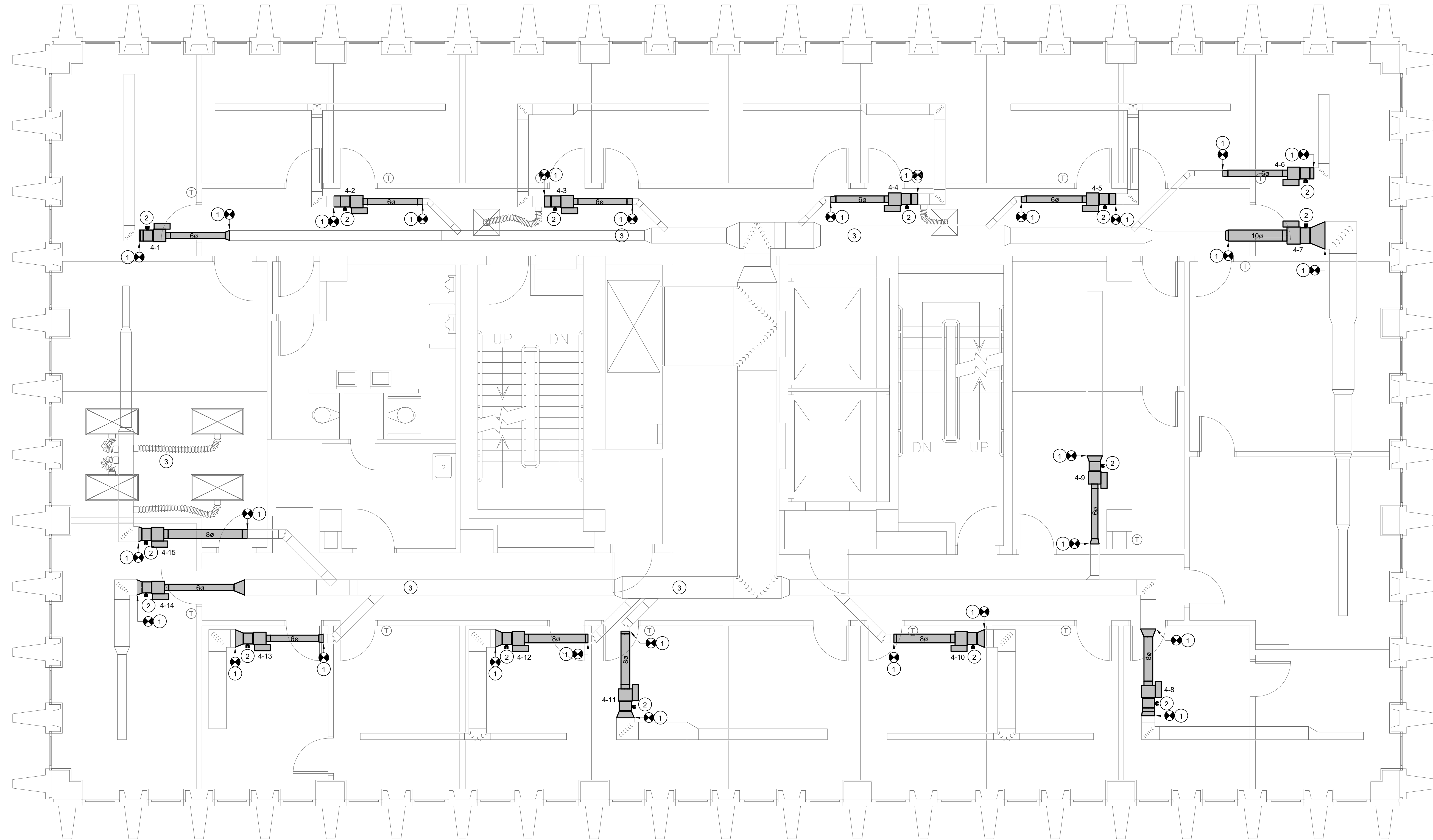
1 FOURTH FLOOR RENOVATION PLAN (ALTERNATE 2) M1 1/4" = 1'-0"
