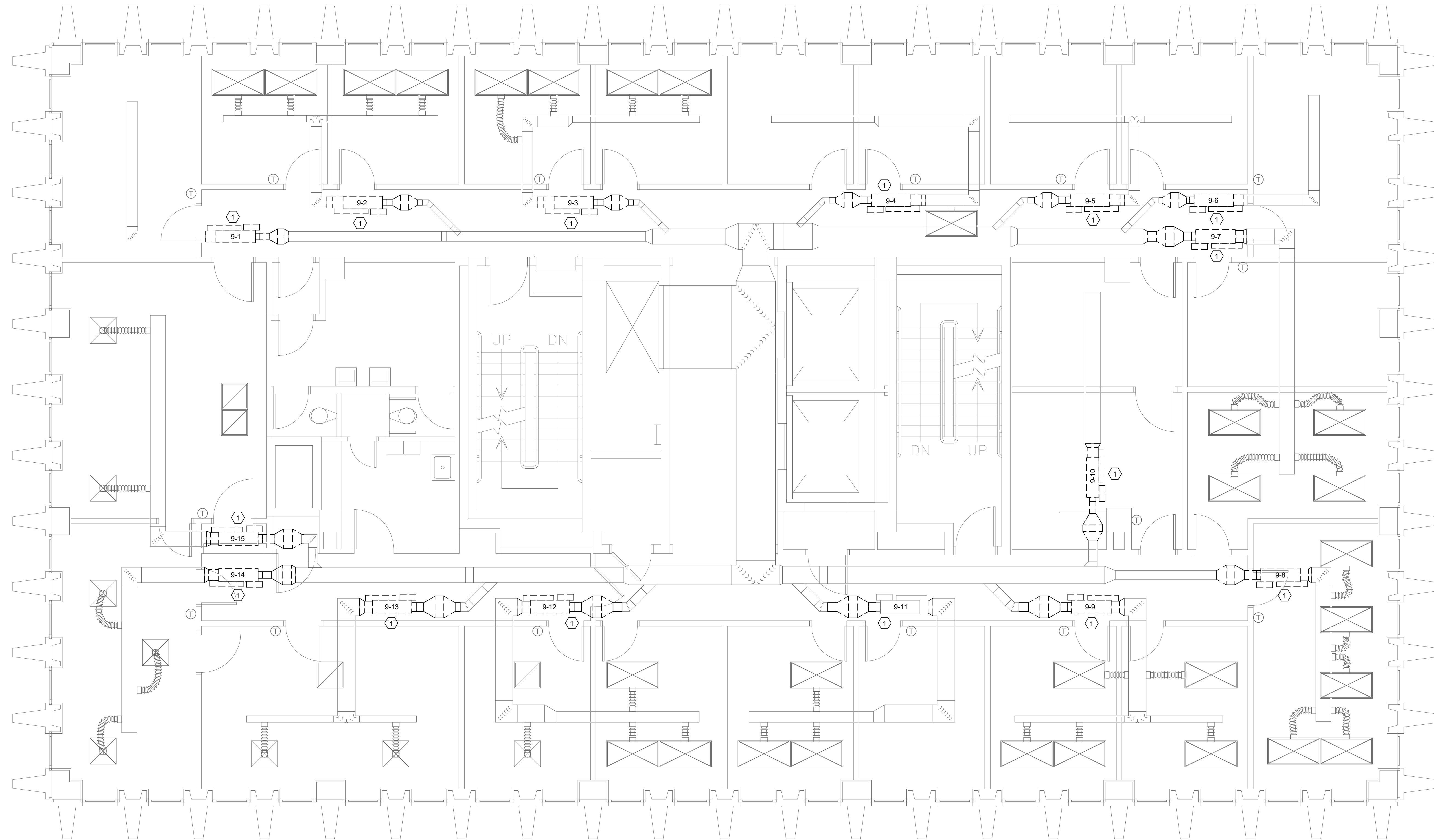
① NINTH FLOOR DEMOLITION PLAN MD6 1/4" = 1'-0"
