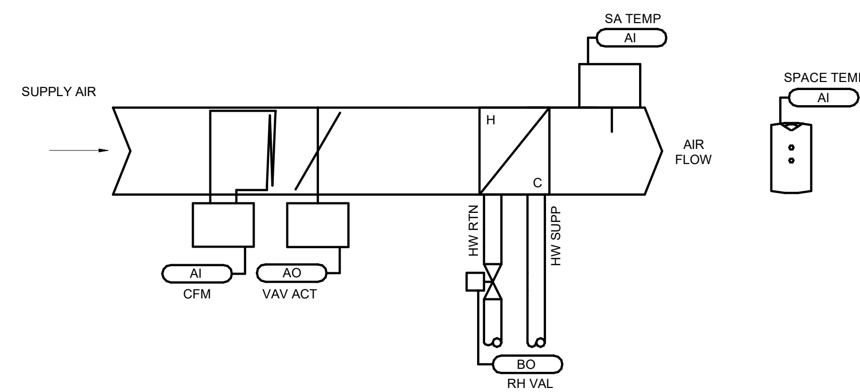
SINGLE DUCT VAV CONTROL DIAGRAM NO SCALE
