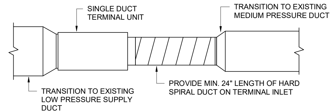
VAV BOX CONNECTION DETAIL NO SCALE
