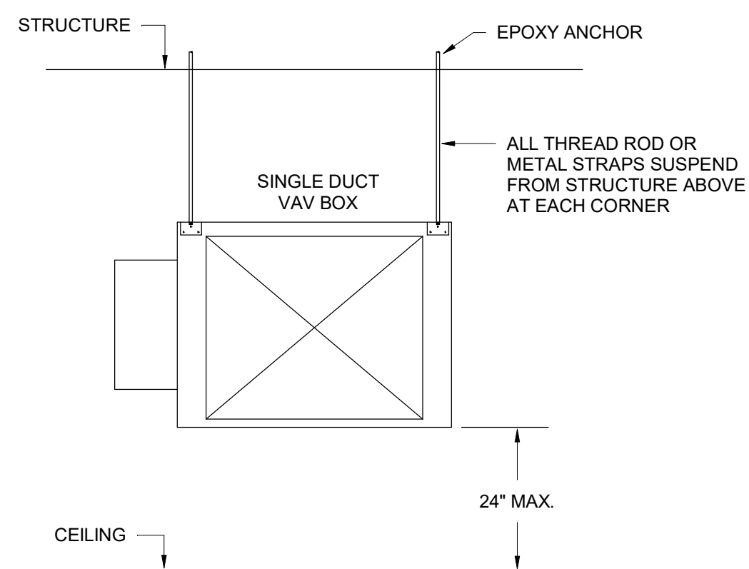
SINGLE DUCT VAV BOX SUPPORT DETAIL NO SCALE
