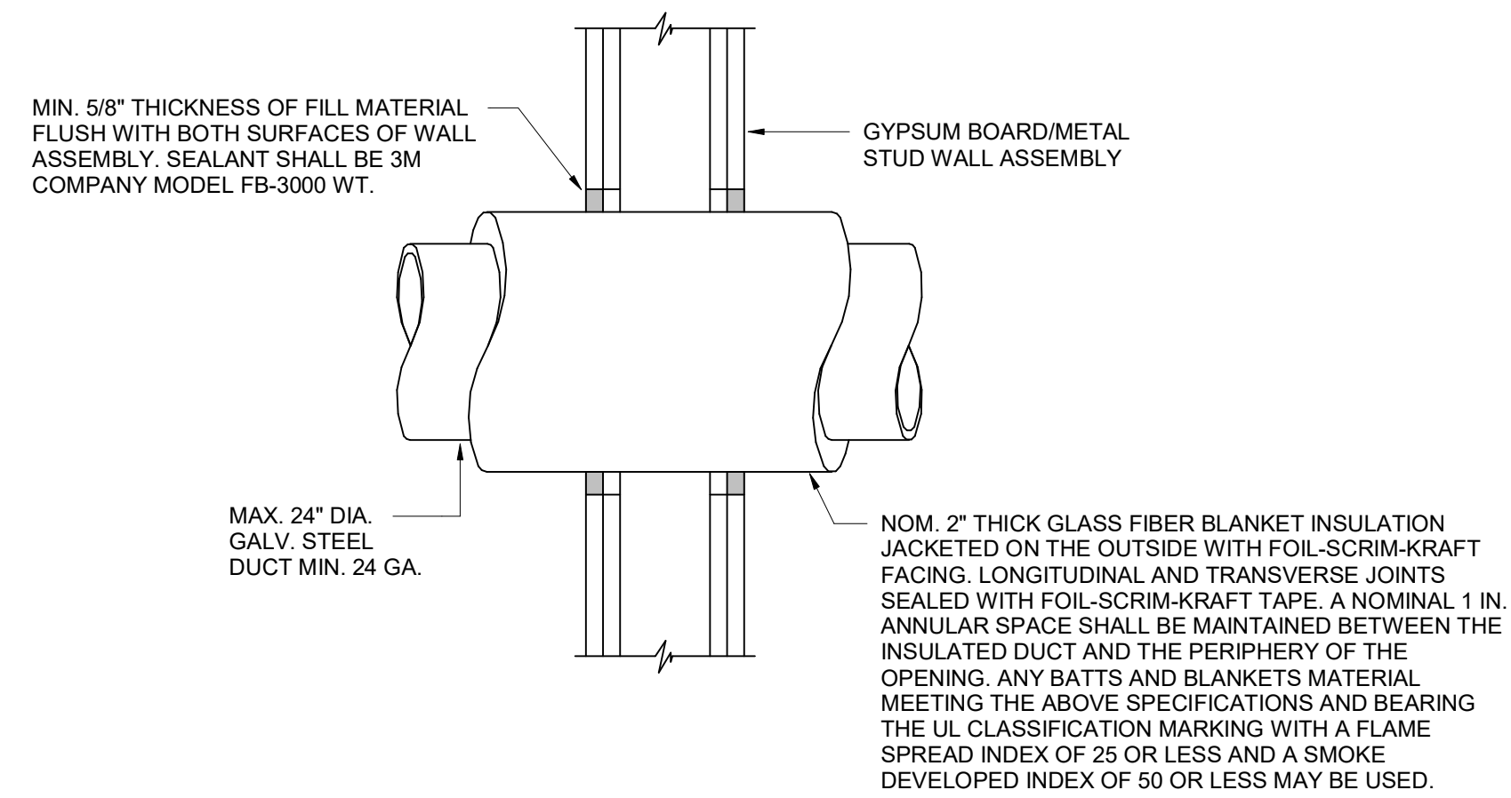
U.L. SYSTEM W-L-7177 DETAIL NO SCALE
